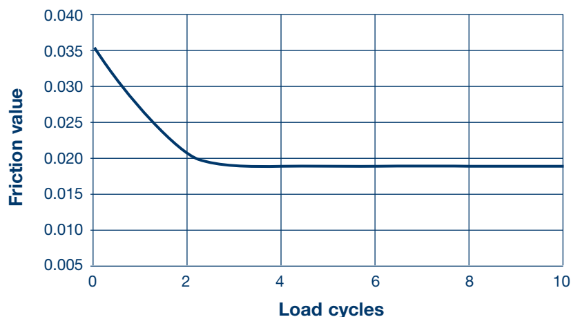
Figure 4: Friction values
