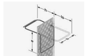
FERBOX® B08/B08S
